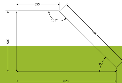
FRISBEE LEFT SIDE student desk
